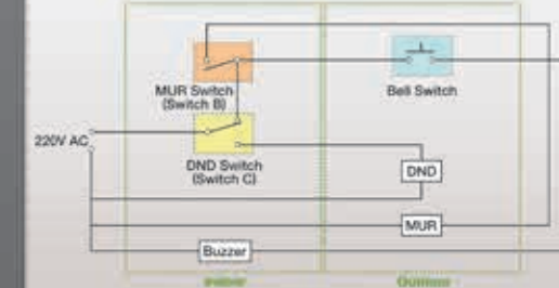
WSBC9220W 1G 3-Way SP (Don't Disturb) 1G 1-Way SP (Make Up Room)
